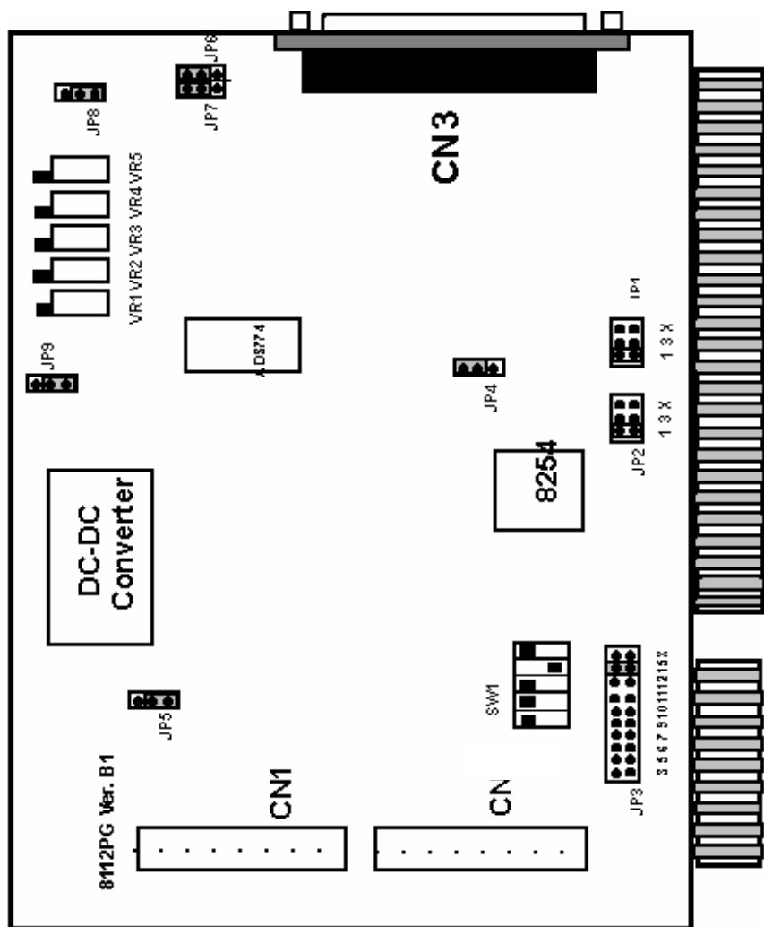
Figure 2.1-2 PCB Layout of the ACL-8112PG
